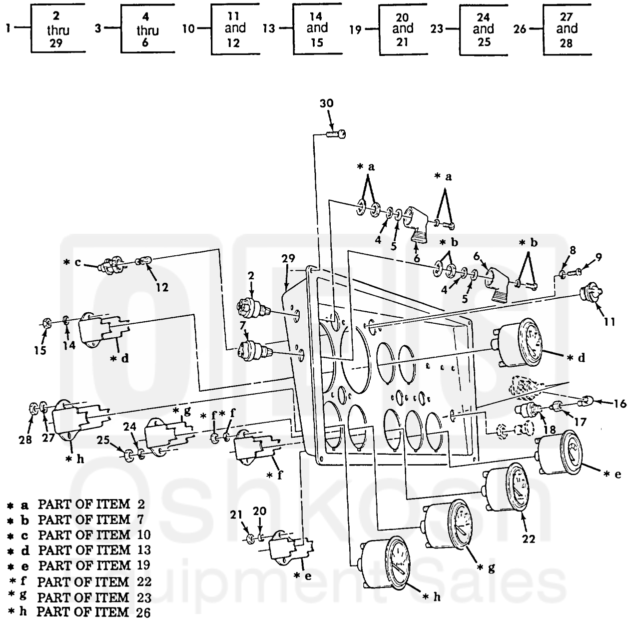
Figure 132. Instrument Cluster Assembly.
